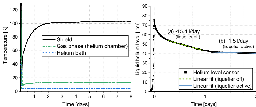
Figure 5.8: (left) Evolution of the temperatures at different sections of the beam-line cryostat in the measurement configuration after helium filling. A nozzle is installed at the helium lifter to reduce the excessive gas circulation. (right) The decline of the helium level measured with a resistive helium level sensor. Section (a) shows the stand-alone evaporation of the cryostat with the basic instrumentation. Section (b) gives the reduced evaporation when the helium re-liquefier is active.
