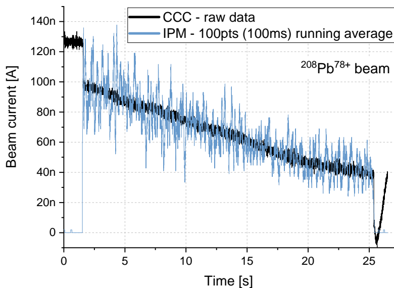
Figure 6.20: Comparative measurement of a stored coasting ^{208}\text{Pb}^{78+} beam by the CCC (unfiltered, black), with R_f = 30\text{ k}\Omega and GBP = 7.2\text{ GHz} , and by the horizontal IPM (averaged, blue). The liquefier was switched off.
