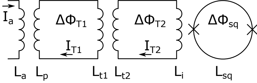
Figure 3.5: Schematic of the 2-stage coupling transformer of a CCC with a large inductance of the pick-up (e.g. due to a high-permeability core).
