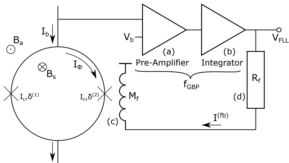
Figure 2.4: Circuit diagram of the FLL readout electronics for a dc SQUID. The FLL feedback scheme linearizes the output of the SQUID to an external flux.
