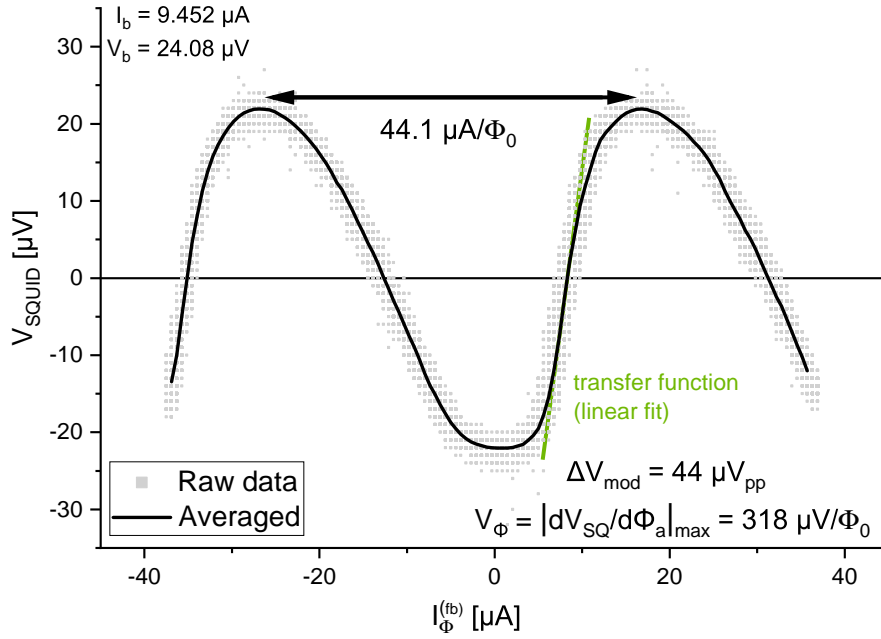
Figure 4.7: The modulation of the voltage across the SQUID V_{sq} with a current through the feedback coil I_{\Phi}^{(fb)} . The bias current I_b is selected such that the transfer function V_{\Phi} (green line) at the working point is maximized. Data collected inside the wide-neck cryostat at GSI.
