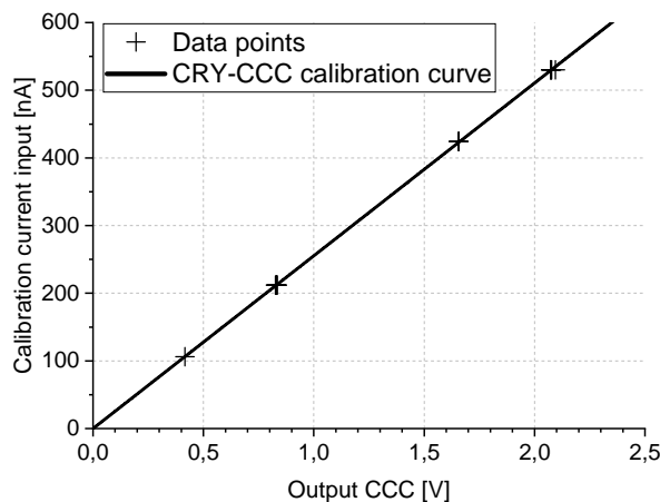
Figure 6.5: Calibration of the CCC inside the beam-line cryostat valid for a feedback resistor \pm 10 V. R_f = 10 k \Omega and for frequencies below 10 kHz.
