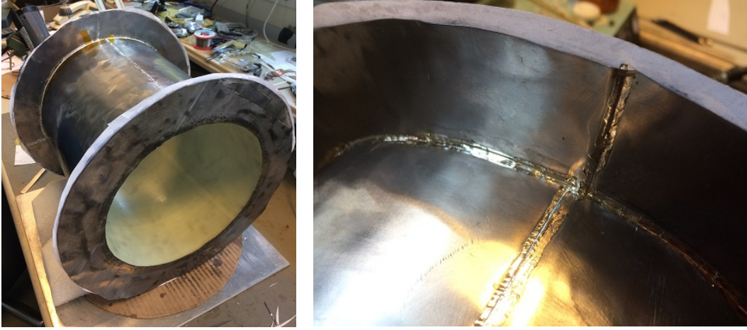
Figure 4.11: Photographs of the CRY-aCCC during the construction. (left) The first screening ring is glued to the inner fiberglass support tube. (right) Close-up view of the soldering connection that has to form a superconducting interface between the lead sheets that is free of any pinholes.
