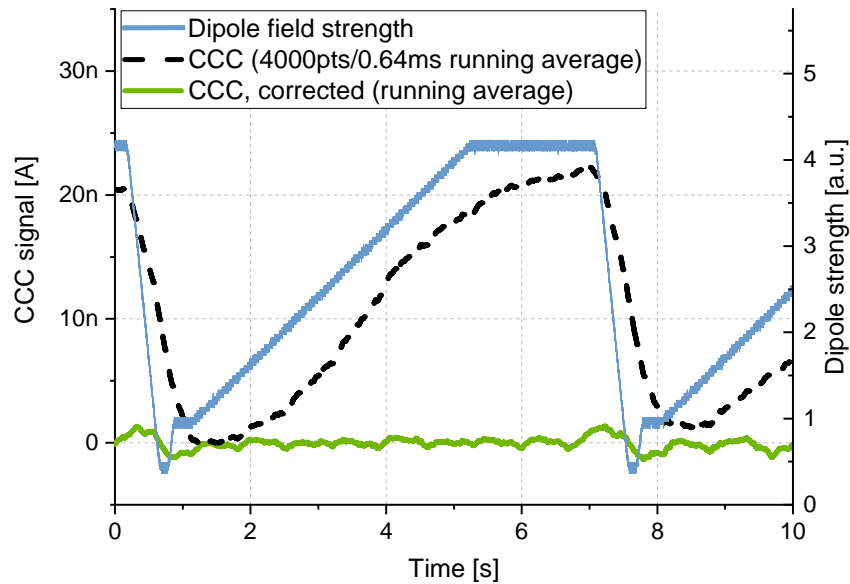
Figure 6.9: The strength of the dipole magnets at CRYRING (blue, right y -axis) measured by a Hall sensor, compared to the resulting background perturbations of the CCC before (dotted black) and after (solid green) the background correction.
