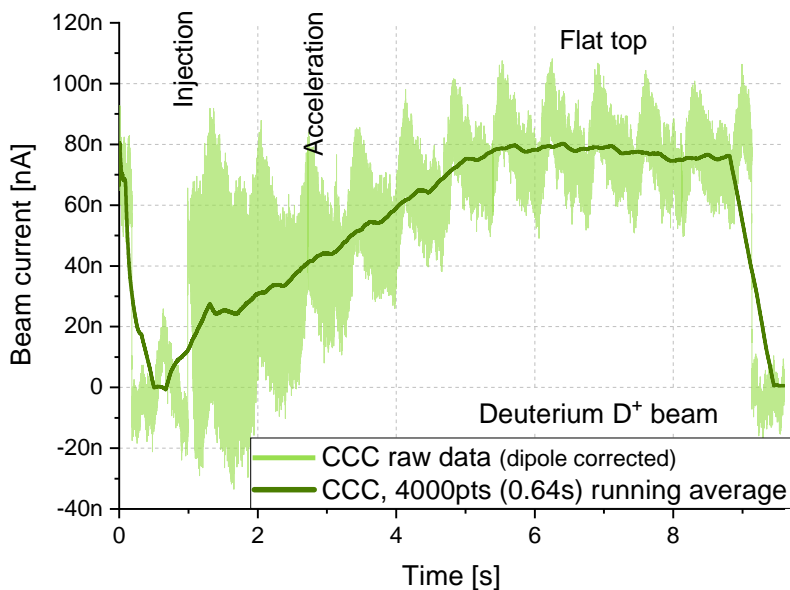
Figure 6.12: Stored, bunched ^2D^+ beam at CRYRING measured by the CCC with an intermediate feedback sensitivity and a large gain-bandwidth-product ( R_f = 7 \text{ k}\Omega , GBP = 5 \text{ GHz} ). The dipole correction was applied. The perturbation by the liquefier is shown.
