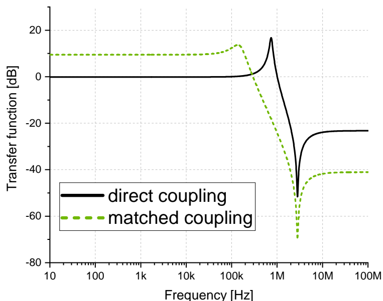
Figure 4.6: The transfer function between the applied (beam) current I_a and the current I_{T2} at the input inductance L_i of the SQUID as a function of frequency simulated with LTspice. The transfer function is given for the direct coupling of the pick-up coil ( L_p = 80 \mu\text{H} ) to the SQUID L_i (solid black) and for the coupling via a flux transformer (dashed green).
