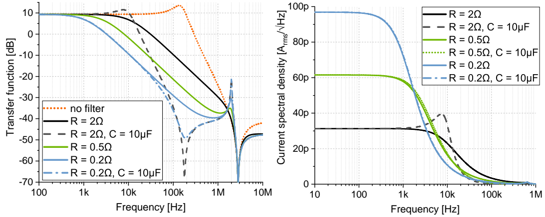
Figure 6.17: The influence of a resistance R_{lp} and a capacity C_{lp} connected to the internal calibration winding on the transfer function (left) and on the noise level due to the thermal noise of the resistor at 4 K (right).
