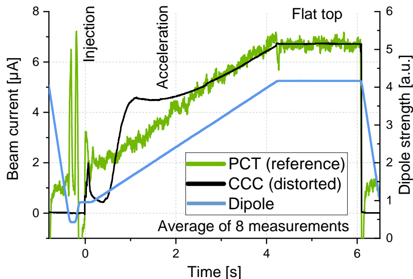
Figure 6.15: Average of eight consecutive measurements of stored bunched {}^2D^+ beam by the CCC (black) with a small feedback resistor and gain-bandwidth-product ( R_f = 0.7\text{ k}\Omega , GBP = 0.23\text{ GHz} ) and by the PCT (green). The field strength of the dipole magnets is given in blue. The voltage output of the PCT was converted to current via the calibration factor 100\ \mu\text{A/V} . After the injection the output of the CCC is distorted due to the large slew rate of the beam current.
