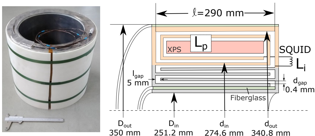
Figure 4.10: (left) Photograph of the coreless CRY-aCCC. (right) Schematic cross section of the axial shield topology. The pick-up coil is highlighted in beige. Not all 12 individual shielding screens are depicted.
