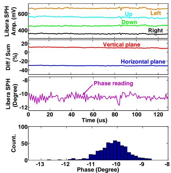
Figure 4: Single plate amplitude, position & phase reading within 1 \mu s time resolution during one macro-pulse. The bottom figure is the histogram of the phase reading.
