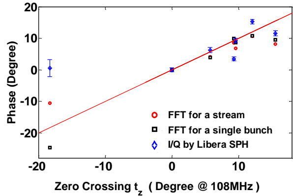
Figure 7: Time-domain data versus Libera SPH and FFT calculations for a single bunch and a stream of bunches.
