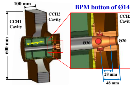
Figure 2: The technical layout of the inter-tank section.
