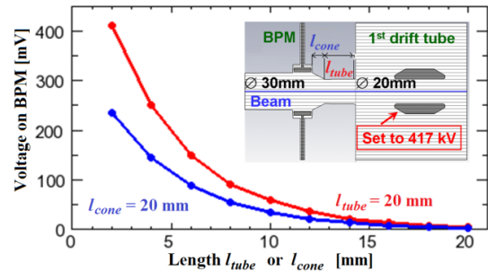
Figure 3: Shielding properties as a function of the length of the cone l_{cone} (red) for a fixed length of the tube or as a function of the cylindrical tube length l_{tube} (blue) for fixed cone length. For the electro-static solver the first drift tube is set to 417 kV.
