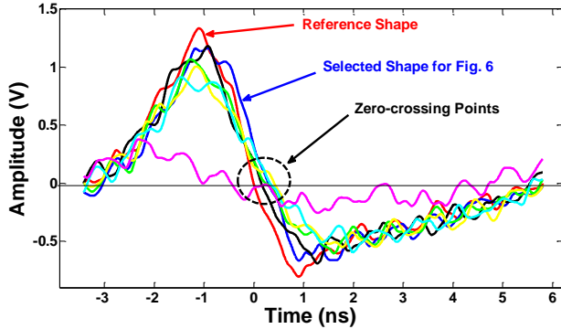
Figure 5: Time-domain recording of single bunches for different buncher amplitudes are depicted to determine the individual zero-crossing points.
