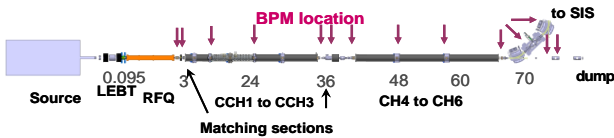
Figure 1: Layout of the proton LINAC including BPM locations.
