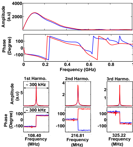
Figure 6: Amplitude and phase spectra for the reference shape (red) and the selected shape (blue) from Fig. 5. (up) from a single bunch, (down) from a stream of bunches (the amplitude spectrum nearly coincided).
