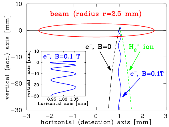
Figure 3.21: Schematic trajectory of an electron in a residual gas monitor with an additional magnetic field on the right. The comparison of the trajectories of an H_2^+ -ion and an electron with and without a magnetic field on the left visualize the broadening due to the beam space charge field. By applying a magnetic field the electron is fixed to the field line, as shown in the insert. The beam parameters are: 10^9 U^{73+} in a 10 m long bunch with radius 2.5 mm.
