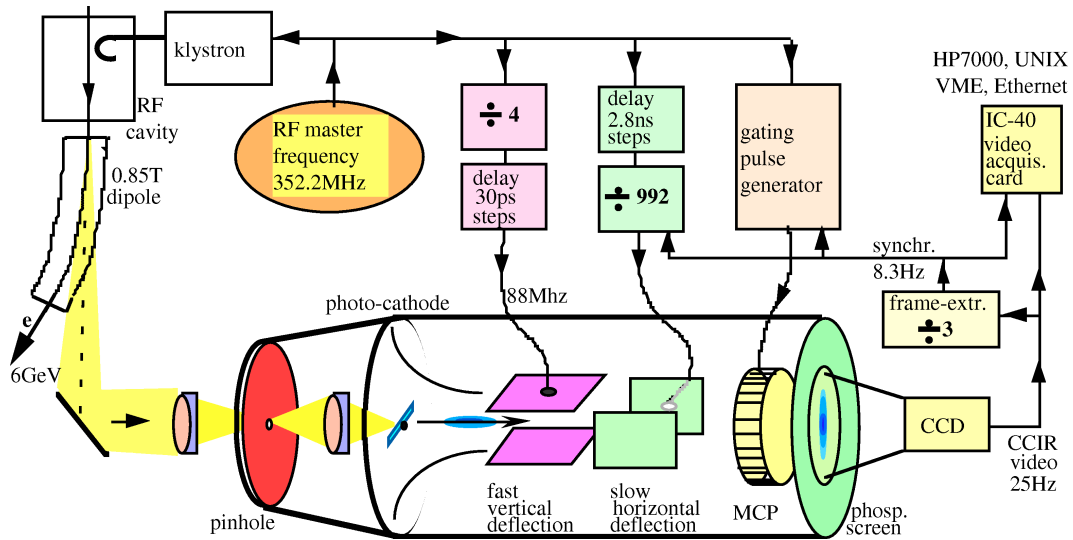
Figure 6.25: Principle of a streak camera measurement for bunch width determination at electron accelerators ESRF, from [118].
