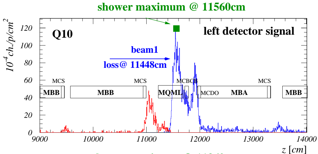
Figure 8.9: Simulation of a secondary particle distribution (hadron shower) due to a proton loss inside a quadrupole for the LHC and 7 TeV protons [134]. The maximum of the shower is about 1 m from the loss point.
