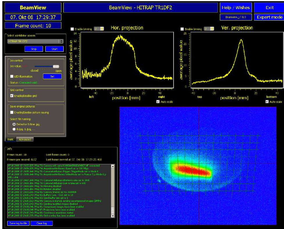
Figure 3.4: Beam spot of a low current 4 MeV/u beam at GSI on a YAG:Ce screen recorded with a digital CCD camera. The original black-white image is converted to false-color for better visibility. The projection on the horizontal axis is shown on the left, the projection to the vertical direction on the right, from [26].
