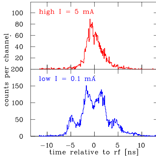
Figure 6.21: The bunch structure measured at the GSI LINAC with a 120 keV/u \text{Ar}^{1+} beam for different currents inside the RFQ [68]. The influence of the beam's space-charge to the longitudinal emittance is demonstrated by it. One rf-period is shown.
