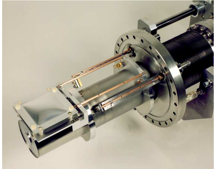
Figure 2.38: Scheme of a SEM (left) and a photo of the SEM part made of 3 Al foils with thickness of 100\ \mu\text{m} of the feed-through used for slow extraction current measurements at GSI.
