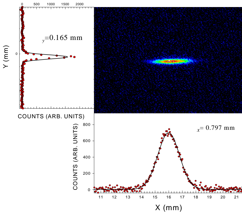
Figure 3.31: Image of the electron beam in the APS accumulator ring (Argonne National Lab.) by a synchrotron radiation monitor [60].
