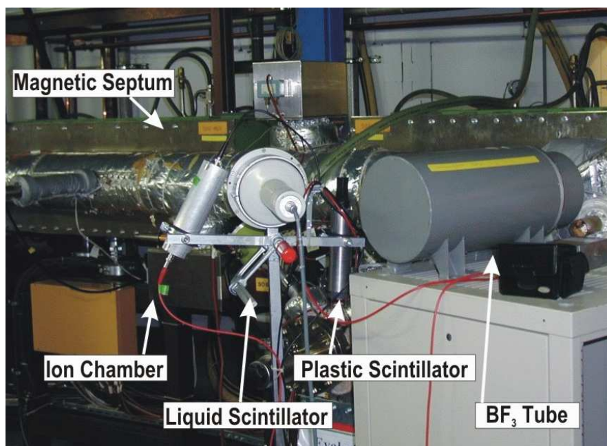
Figure 8.2: The tested beam loss detectors installed at the extraction from the GSI heavy ion synchrotron [130].
