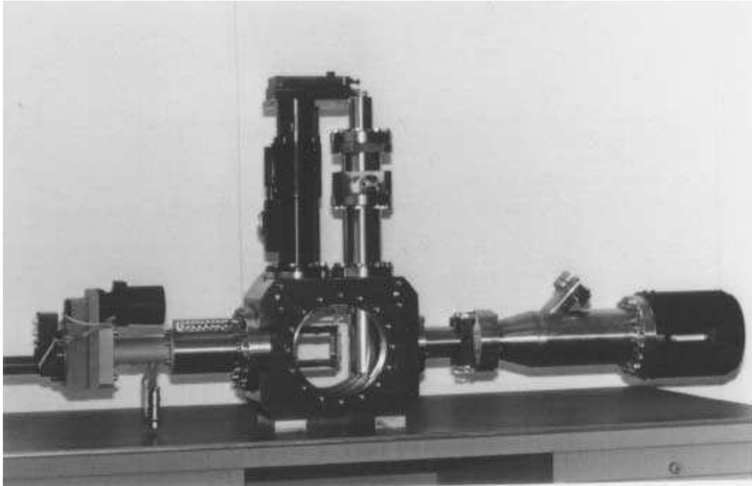
Figure 6.24: The bunch shape monitor (BSM) installed at CERN LINAC 2 [114]. The vacuum feed-through on the left side is the support for the high voltage wire. The rf-deflector is installed on the vertical flange and the detector is mounted on the right.
