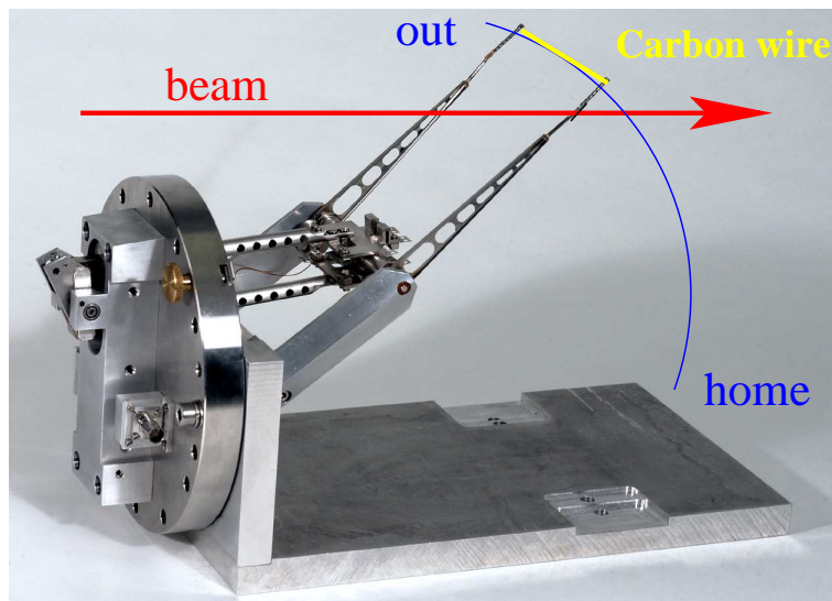
Figure 3.10: Pendulum scanner or 'flying wire' used at CERN synchrotron [28].
