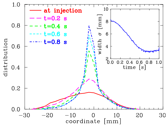
Figure 3.19: The profile during an electron cooling cooling process for an 11 MeV/u Ar^{18+} beam at the GSI synchrotron. Five profiles from the injection (broad peak bottom) to the maximal cooled profile recorded at different time during the cycle. The inset shows the standard deviation of the profile as a function of time.
