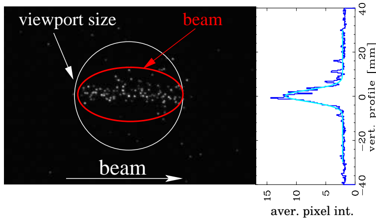
Figure 3.24: Image of a 250 \mu\text{s} \text{Ar}^{10+} beam of I_{\text{beam}} = 2.5 \text{ mA} and a vacuum pressure of 10^{-5} mbar recorded at the GSI LINAC. The original image (recorded with a double MCP intensifier) is shown and the projection for the vertical profile [48].
