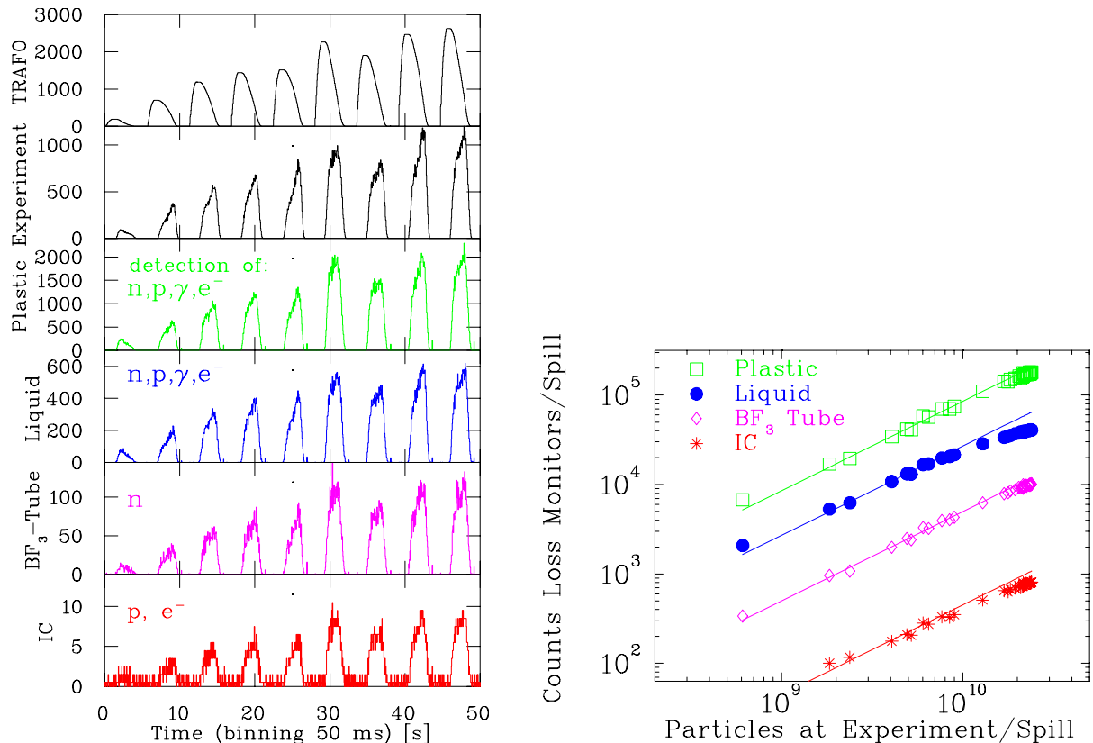
Figure 8.8: Left: Typical example from different beam loss monitors for a O^{8+} beam accelerated from 11 to 800 MeV/u with up to 4 \times 10^{10} particles per spill [130]. Right: Linearity of the loss monitors as a function of the current for the same parameters. The lines are linear fits.
