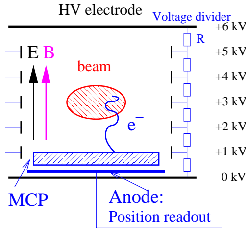
Figure 3.21: Schematic trajectory of an electron in a residual gas monitor with an additional magnetic field on the right. The comparison of the trajectories of an H_2^+ -ion and an electron with and without a magnetic field on the left visualize the broadening due to the beam space charge field. By applying a magnetic field the electron is fixed to the field line, as shown in the insert. The beam parameters are: 10^9 U^{73+} in a 10 m long bunch with radius 2.5 mm.
