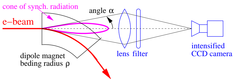
Figure 3.28: Scheme for a synchrotron radiation profile monitor observing the radiation from a dipole.
