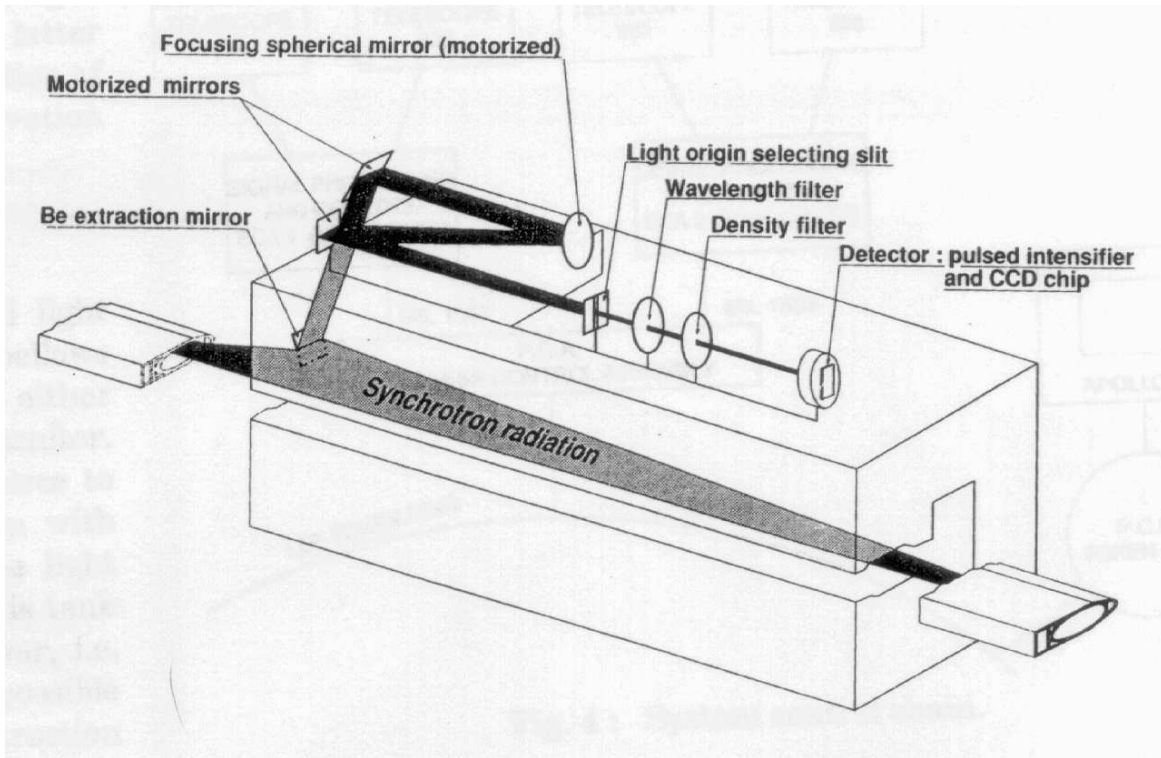
Figure 3.30: The synchrotron radiation profile monitor at LEP. The optical system is installed close to the 23 m long dipole magnet with bending radius of 3100 m, from [59]
