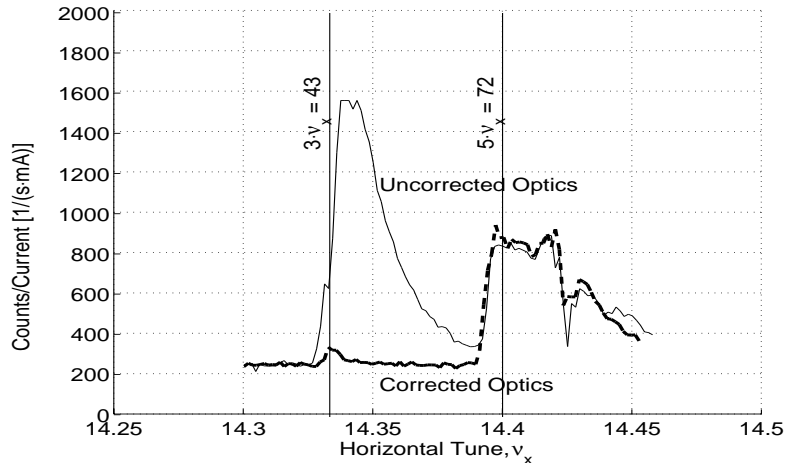
Figure 8.11: Tune scan at the ALS synchrotron light source [136]. For a fixed vertical tune, the horizontal tune is varied and the loss rate, as measured with a scintillator at a collimator is plotted. By changing the setting of some quadrupole, one resonance ( 3 \cdot \nu_x ) can be avoided.
