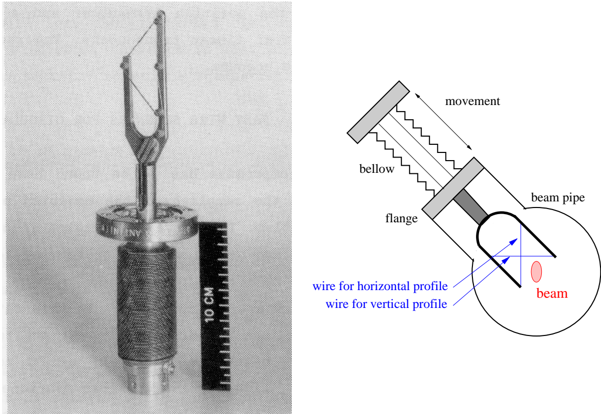
Figure 3.12: Linear scanner used at CERN [31].
