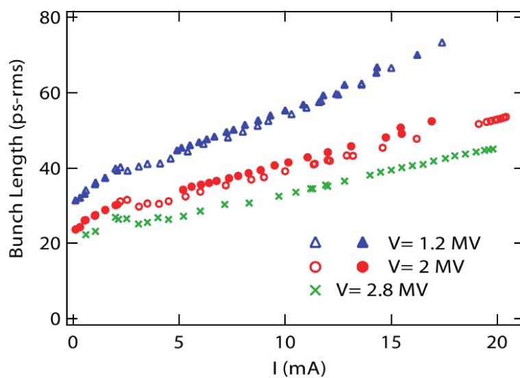
Figure 6.27: Example of the use of a streak camera at the synchrotron light facility SOLEIL achieved from measurements like depicted in Fig 6.26: The bunch-length is recorded as a function of the current for different accelerating voltages [119].
