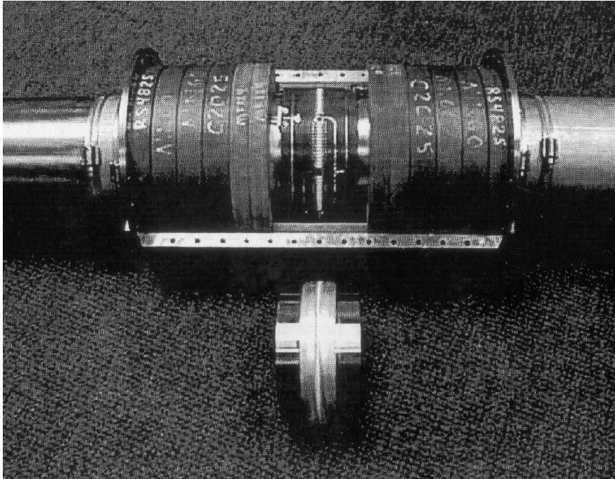
Figure 6.14: Photo of the wall current monitor used at FERMI-Lab for protons, from [109]. The ceramic gap is shown separately. The ferrite rings and the printed circuit with the resistors are visible.
