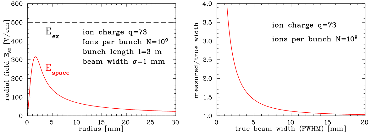
Figure 3.20: Model calculation of the beam broadening due to the space charge field of a U^{73+} with 10^9 particles per 3 m bunch length (left). The resulting relative broadening using a residual gas monitor with ion detection (right) is plotted for this current. The parameters are valid for an intense, cooled ion beam.
