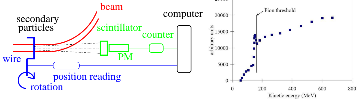
Figure 3.11: Left: Scheme of a wire scanner using the production of secondary particles as the signal source. Right: The total rate from a wire scanner under proton impact at CERN PS-Booster, showing the rate increase above the \pi -threshold at \sim 150 \text{ MeV} , from [30].
