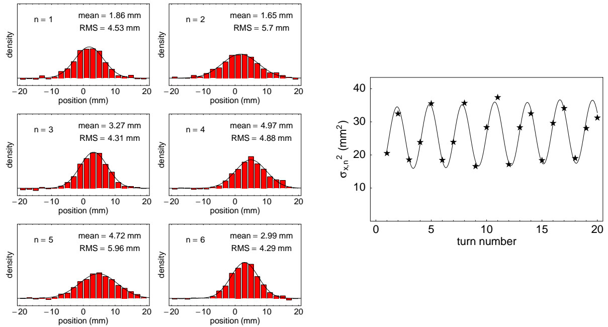
Figure 3.9: Profile measurement for a mismatched injection into the CERN PS synchrotron for the first n = 1..6 turns and the fitted square of the beam width as a function of time, from [34].
