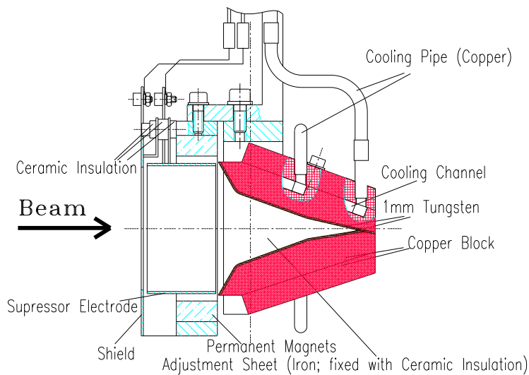
Figure 2.27: A Faraday cup and beam stopper of high intensity beams as installed at the high current LINAC at GSI. The opening of the cup is \varnothing 50 mm
