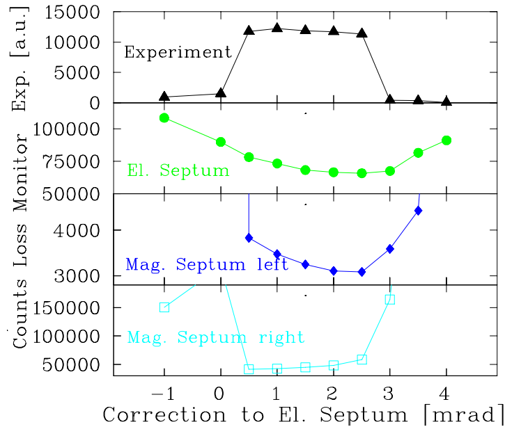
Figure 8.10: Counts per spill from three loss monitor locations and the current at the experiment as a function of the angle electrostatic septum at the GSI synchrotron [130].
