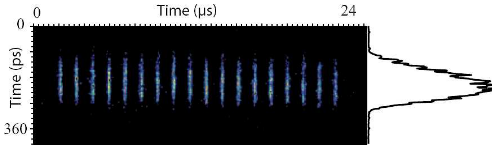
Figure 6.26: Bunch length measurement with a streak camera, using synchrotron light from a dipole at SOLEIL [119]. The horizontal axis scaling is 24 \mu\text{s} for the bunch repetition and the vertical axis is 360 \text{ ps} full scale for the bunch structure. The bunch width is \sigma \simeq 40 \text{ ps} as achieved for a medium current of 12 \text{ mA} and a rf-voltage of 2 \text{ MV} , see Fig. 6.27 for a compilation of such measurements.
