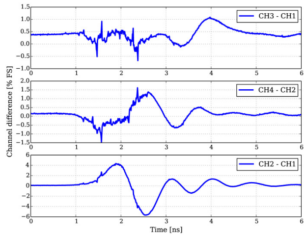
Figure 2: Measurement of oscilloscope channel symmetry. Shown are relative differences of the waveforms of Fig. 1.
