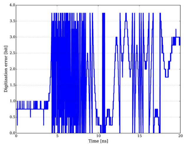
Figure 5: 8-bit dataset computed from the 12-bit dataset for the 1.2 ns pulse (top). Bits of error per sample of the 8-bit dataset obtained by comparing it to the 12-bit data (bottom).
