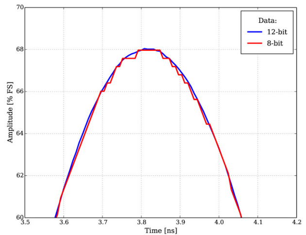
Figure 3: Comparison of the same signal with 12-bit and 8-bit resolution, zoom on the top of the pulse.
