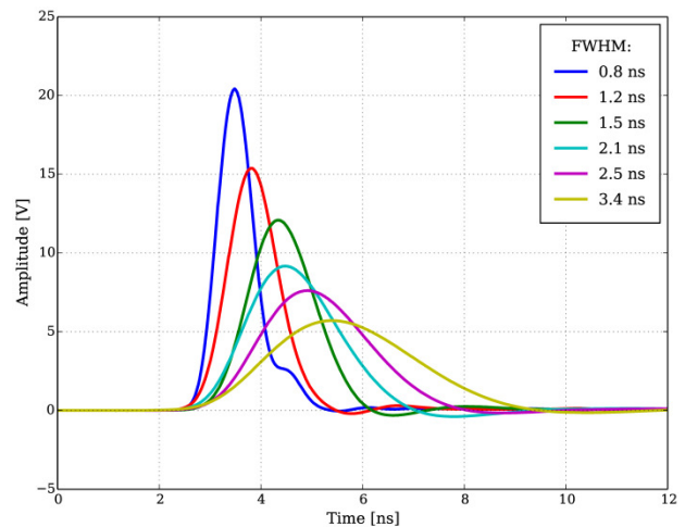
Figure 4: Pulses undergoing digital integration. The 0.8 ns pulse comes directly from the avalanche generator and the other pulses were produced using low-pass filters.
